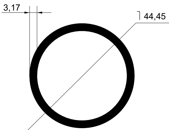
TUB-399 A 1,120 kg/m
